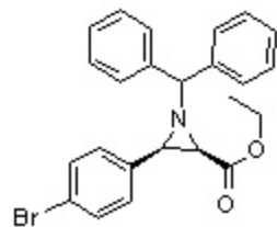
(2R,3R)-ethyl 1-benzhydryl-3-(4-bromophenyl)aziridine-2-carboxylate
