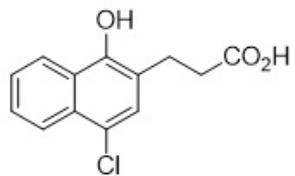
2 Molecular Weight: 250.678
