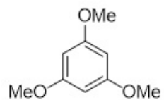
1,3,5-trimethoxybenzene ( TMB ), Internal standard, Molecular Weight: 168.192
